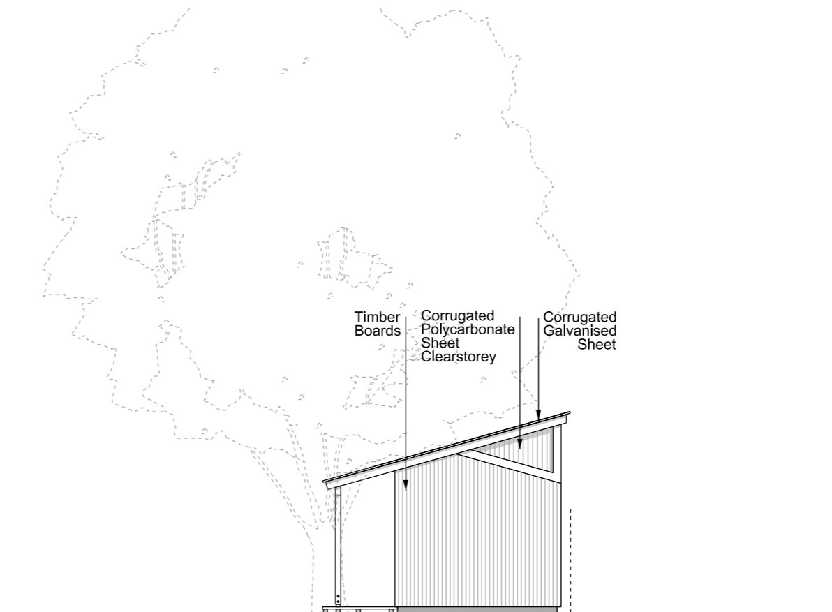
04 0207 Proposed Elevations Animal Enclosure 1:100@A3
